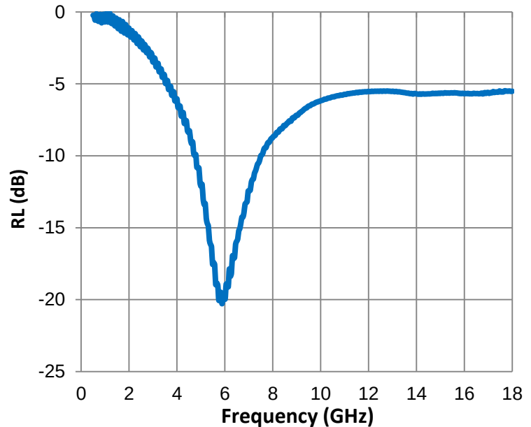
Reflection Loss
