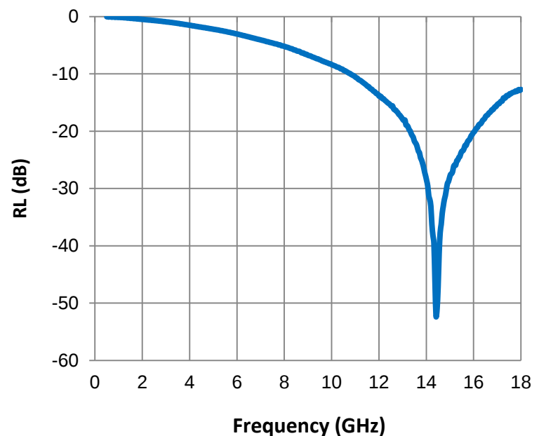
Reflection Loss
